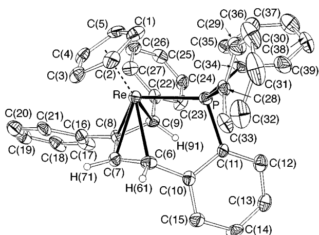
Fig. 7 Molecular structure of [\text{Re}\{\eta^4\text{-CH(Ph)=C(Ph)CH=CHC}_6\text{H}_4\text{-PPh}_2\text{-}o\}(\eta\text{-C}_5\text{H}_5)] 10
