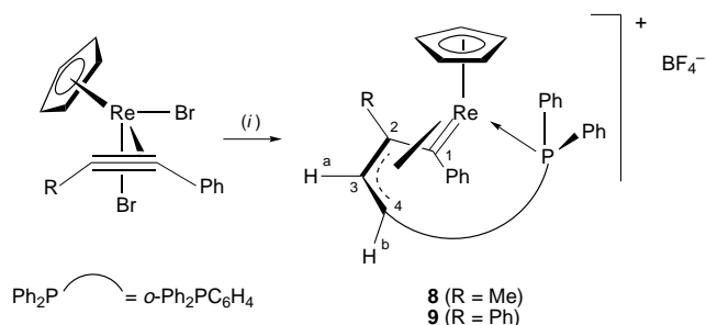
Scheme 6 (i) dppe, 2AgBF 4 , thf, -2AgBr, -HBF 4
