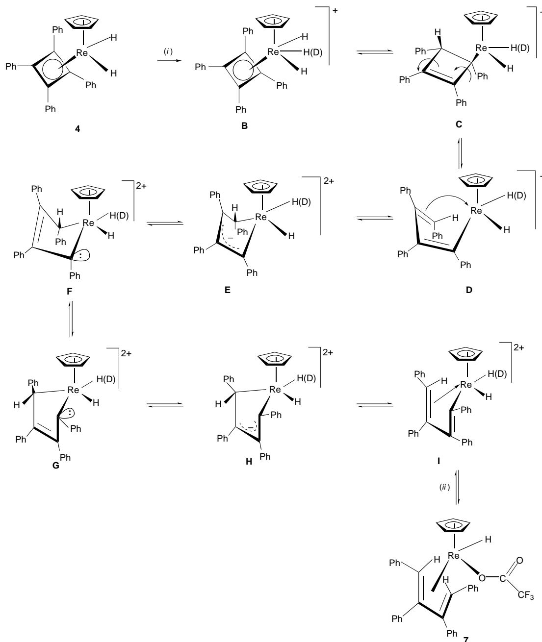
Scheme 4 (i) + \text{CF}_3\text{CO}_2\text{H(D)} , (ii) + \text{CF}_3\text{CO}_2^-
