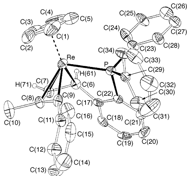
Fig. 5 Molecular structure of the cation present in the complex [Re{C(Ph)-η 3 -C(Me)CHCHC 6 H 4 PPh 2 -o}(η-C 5 H 5 )] [BF 4 ] + 8
